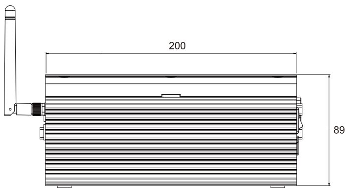
Side view (with optional Wi-Fi antennas)
