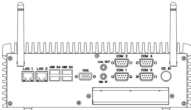
Rear view (with optional Wi-Fi antennas)
