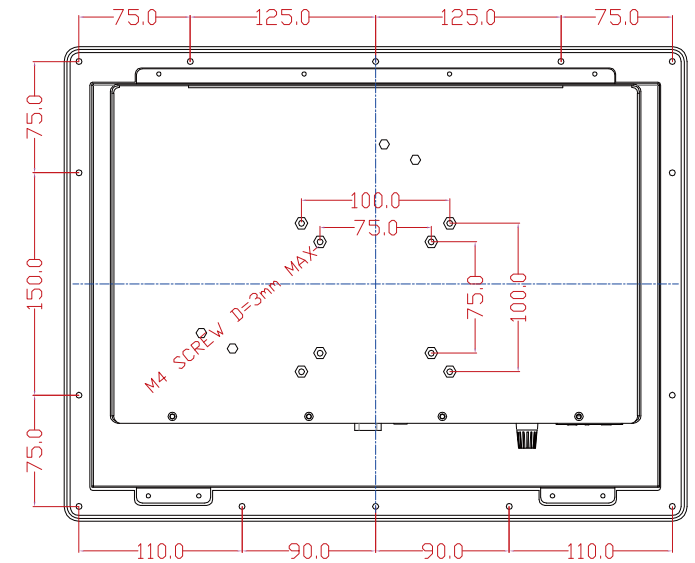
MOUNTING CUTOUT DIMENSIONS: 388 × 280 mm
