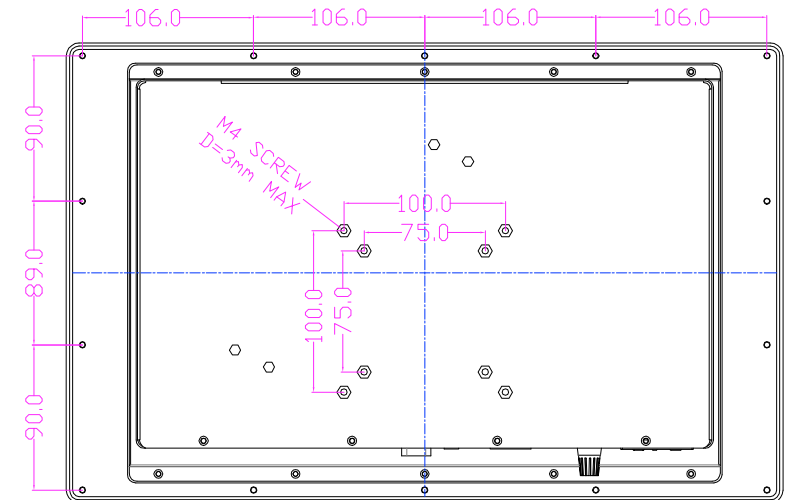
MOUNTING CUTOUT DIMENSIONS: 370 × 245 mm
